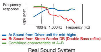
Stream Woofer DB (Double Bass-reflex)
